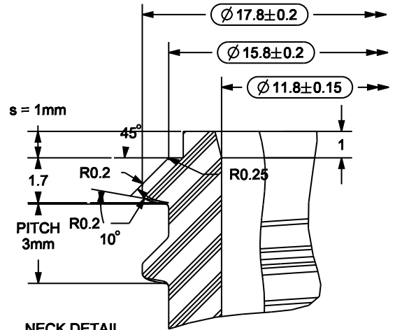
NECK DETAIL SECTION X-X SCALE 5:1
