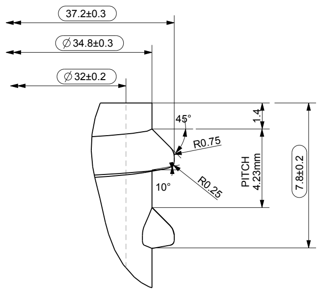
DETAIL ON THREAD SCALE 5:1 NECK FINISH SP-400 M38
